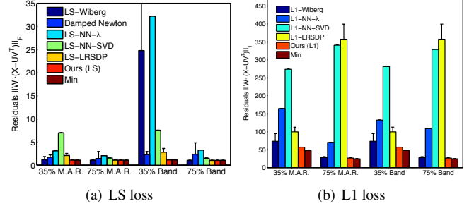
Figure 4. Comparison of convergence to empirical global minima (Min) for the LS and L1 losses in synthetic data. The minima are found as the minimum of all 100 runs of all methods for each test.
